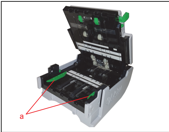
Figure 1 iVIZION Validator Head (with Guides) (P/N 251870)
