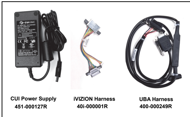
Figure 1 Power Supply Kit for iVIZION® and UBA®
