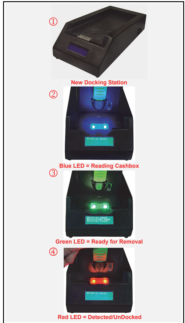
Docking Station LED Indications
