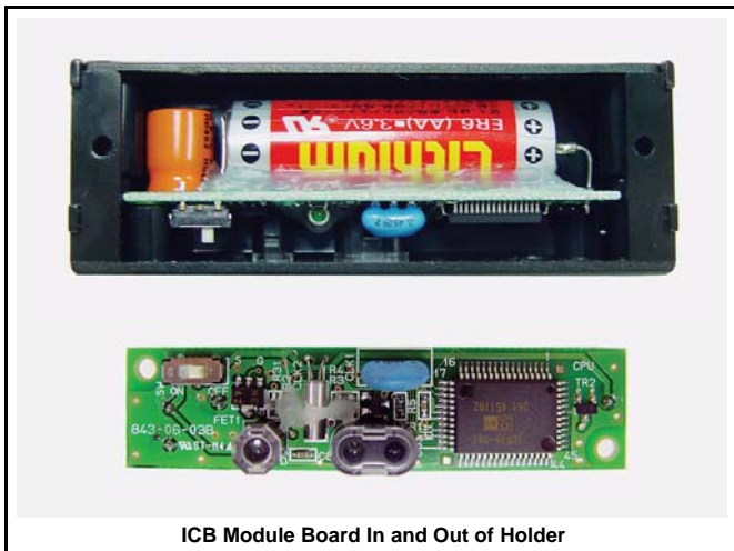
ICB Module Board In and Out of Holder
